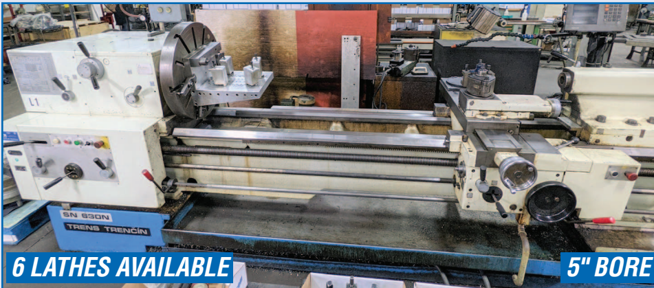
TOS SN 630N GAP BED ENGINE LATHE
